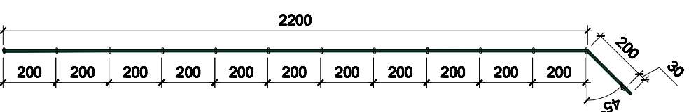
Sections (All heights shown) SCALE: 1:20@A3
