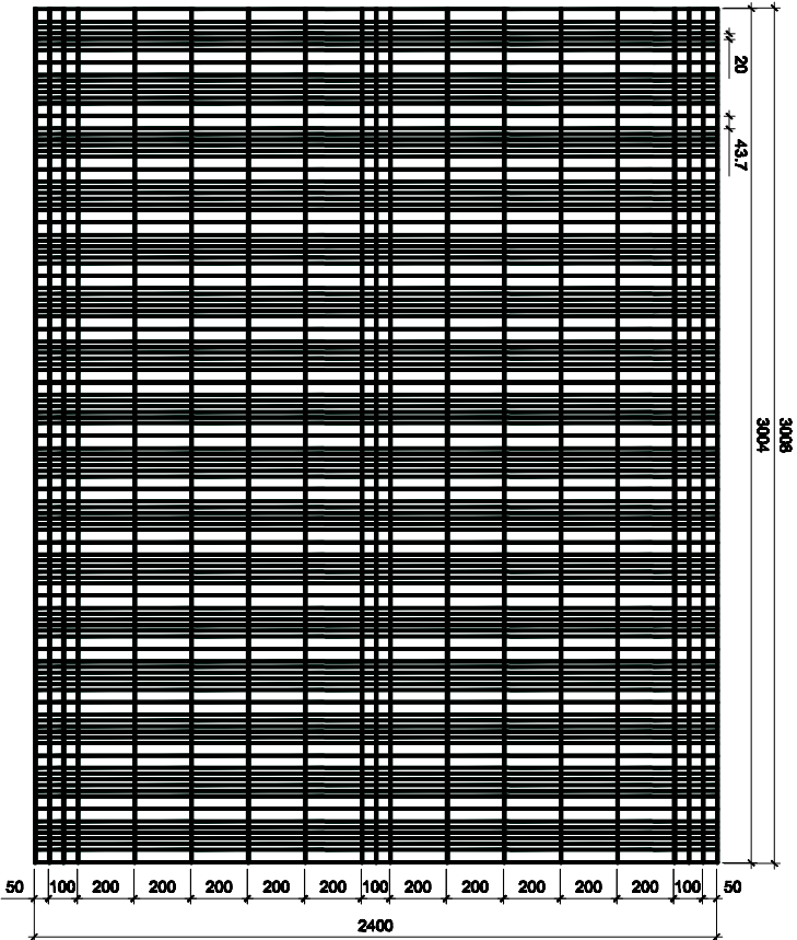
Elevation (2430 high panel) SCALE: 1:1000
