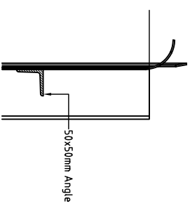
RAIL VIEWS scale 1/10
