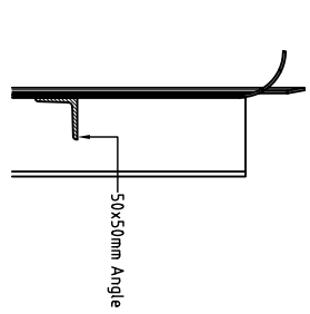
RAIL VIEWS scale 1/10
