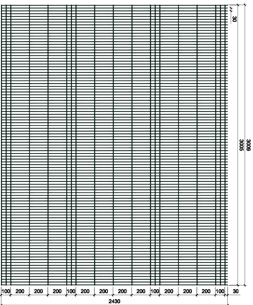
Elevation (2430 high panel) SCALE: 1:120@A3
