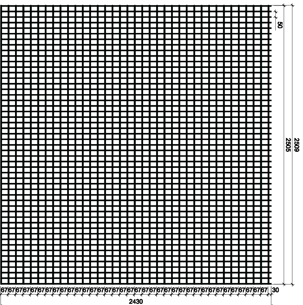
Elevation (2430 high panel) SCALE: 1:200@A3
