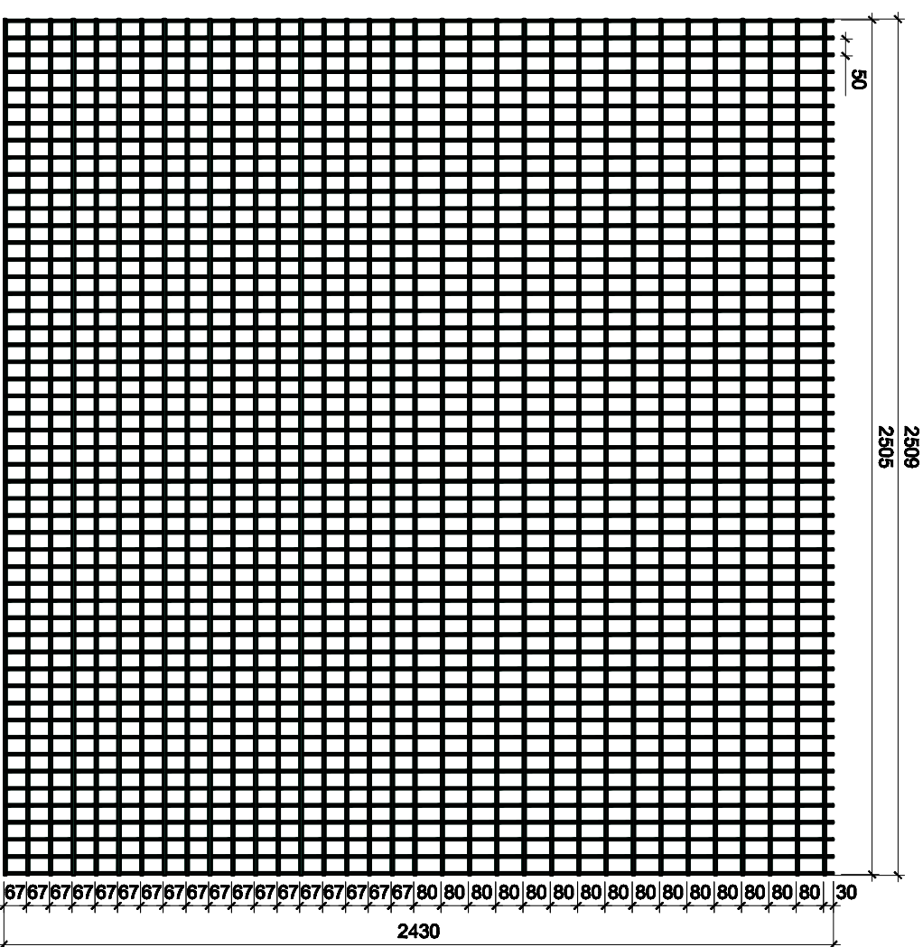
Elevation (2430 high panel) SCALE: 1:200@A3
