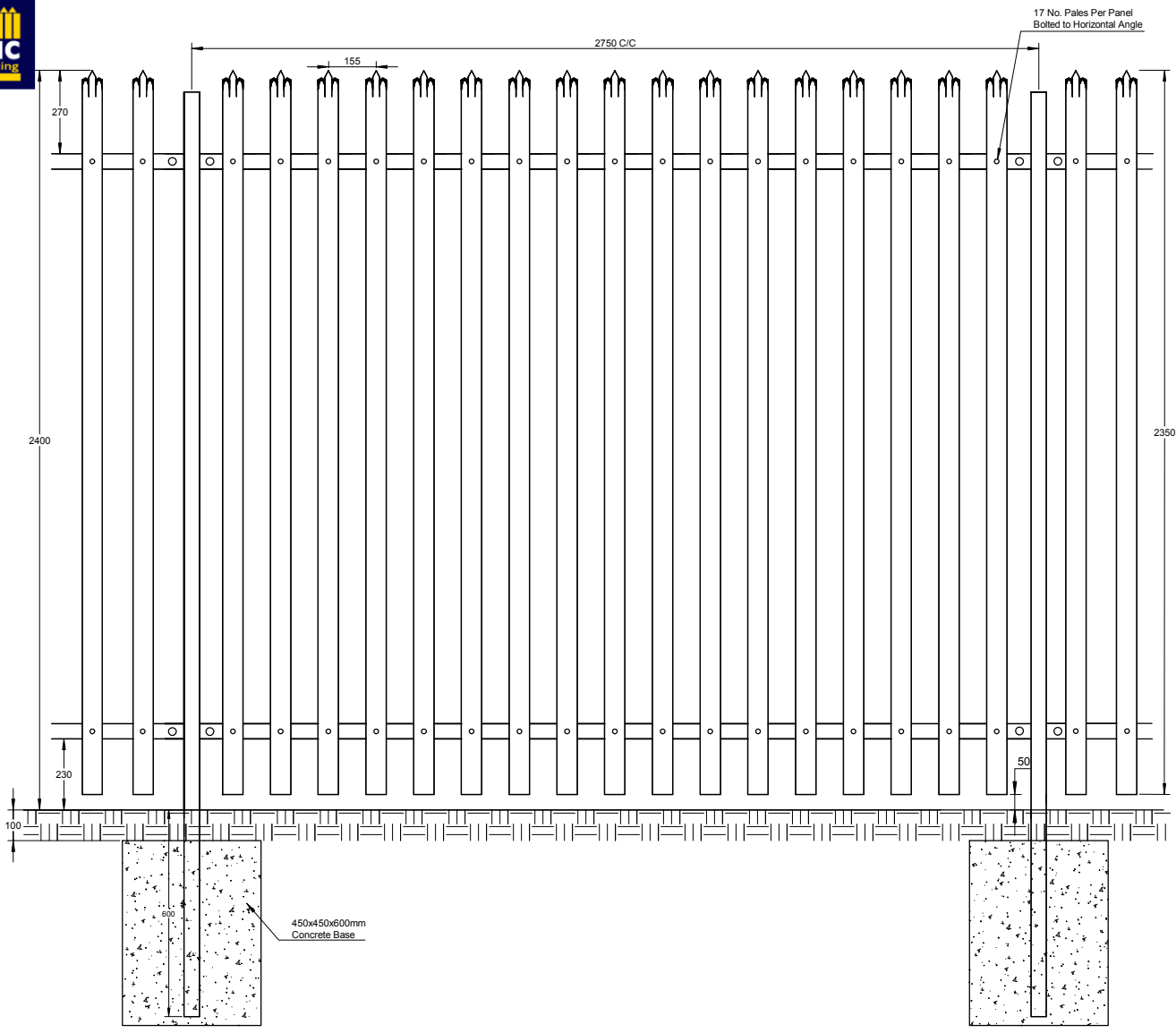
Front Elevation
