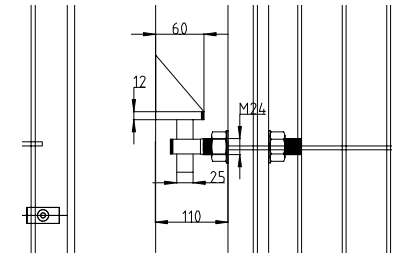
HINGE DETAIL
