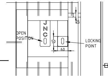
LOCK DETAIL
