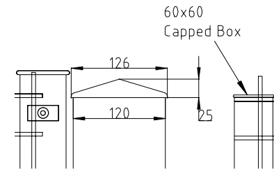
POST CAP DETAIL
