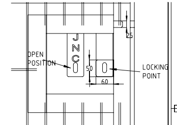
LOCK DETAIL
