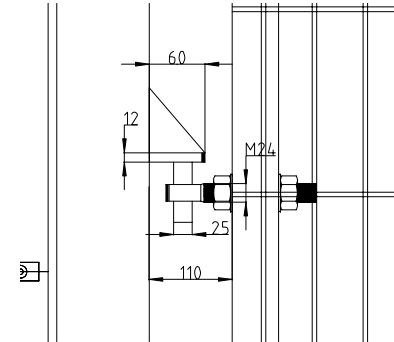
HINGE DETAIL
