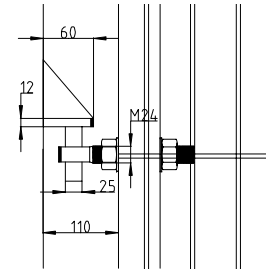
HINGE DETAIL
