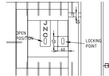
LOCK DETAIL
