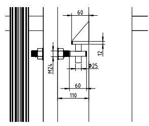
HINGE DETAIL scale 1/10
