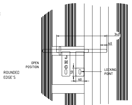
LOCK DETAIL scale 1/10
