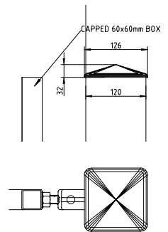
POST CAP DETAIL scale 1/10
