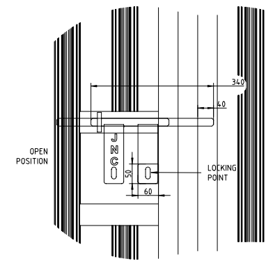
LOCK DETAIL scale 1/10
