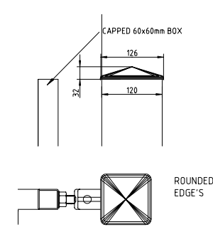
POST CAP DETAIL scale 1/10
