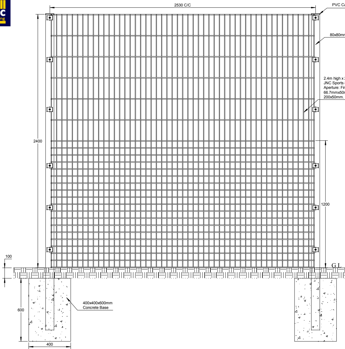
Front Elevation
