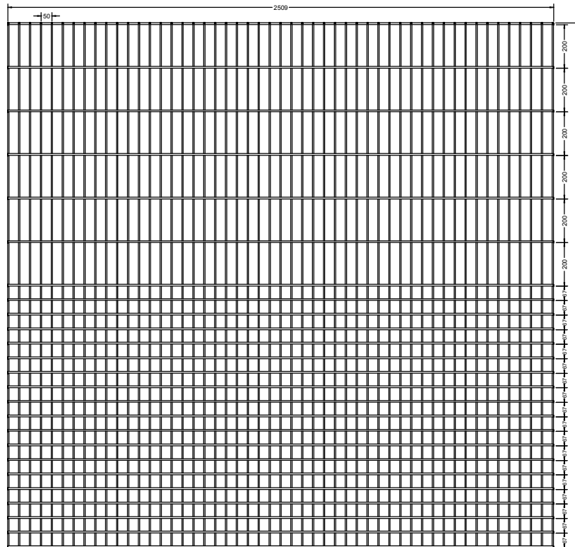
Elevation (2400 high panel)
