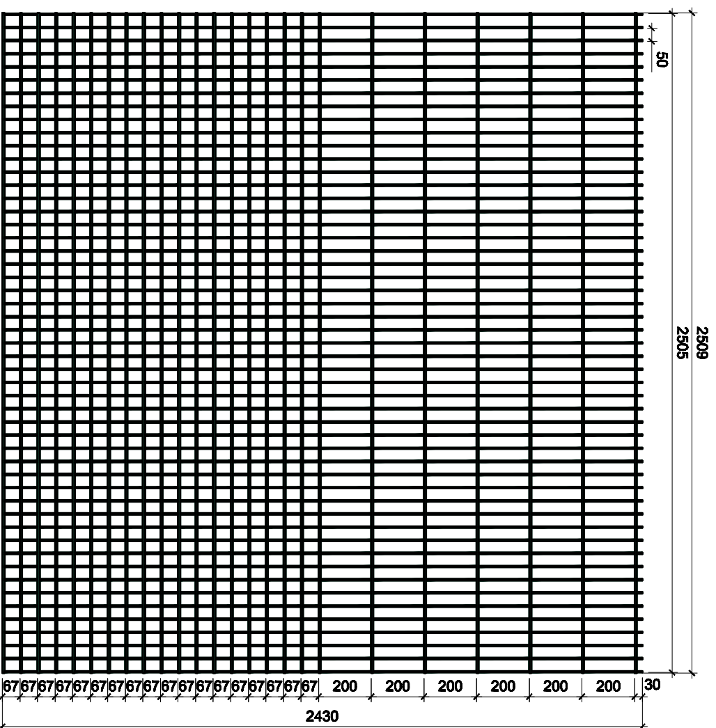
Elevation (2430 high panel) SCALE: 1:120@A3
